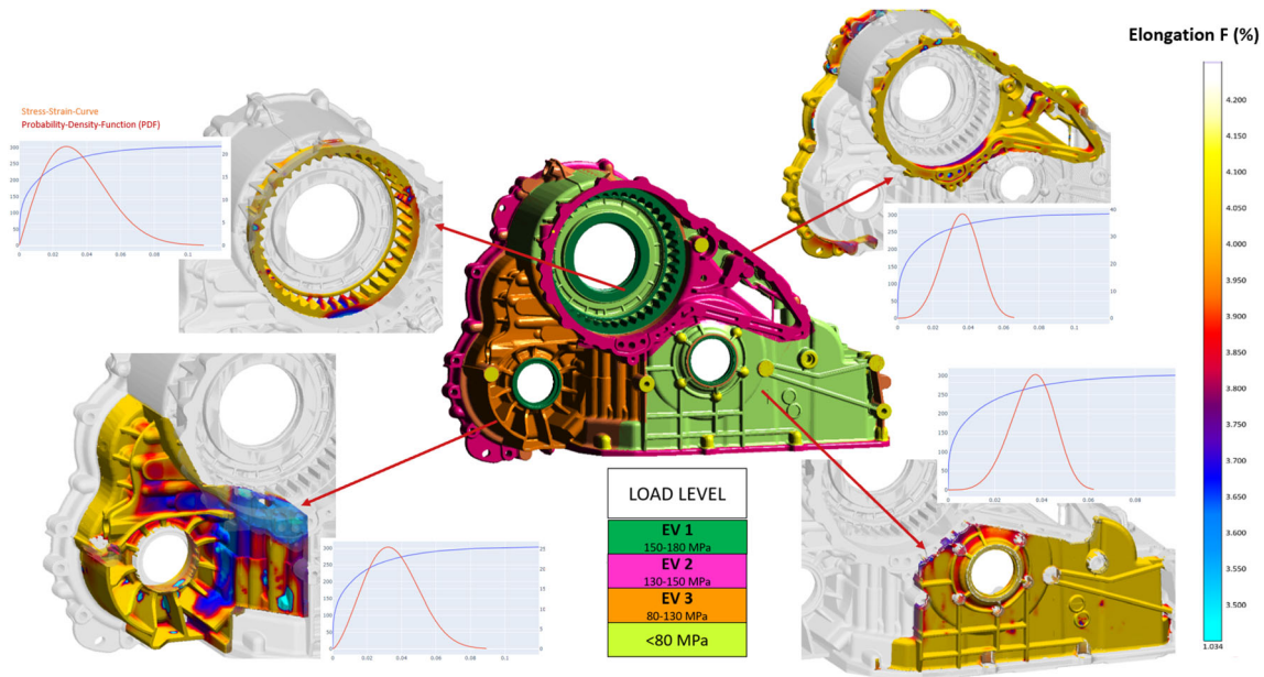
Figure 22. The methodology is applied to different zones within the casting, each with unique requirements. The curves illustrate the expected stress-strain curve and the distributions of mechanical properties at the statistical mean of each zone. The probability function is fed by the initially defined process variability, the locally predicted ideal mechanical properties and the statistical evaluation of simulated defects or other quality criteria in any zone.
