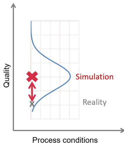
Figure 9. Deviation between simulation and reality. Apparent discrepancies between the results of a simulation and an observed defect can often be explained by different probabilities.
