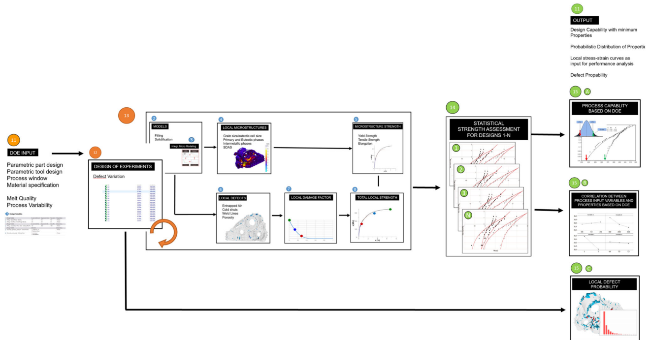
Figure 23. Flow chart of the overall process for determining process capability. Instead of a single simulation, the methodology is supplemented by a virtual test plan in commercial software, in which all process parameters are systematically examined and evaluated.
