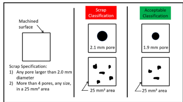
Figure 7. Specification of reasons for rejections in the casting. The smallest fluctuations in the measured error variables can lead to rejects, depending on the limit value. 28
