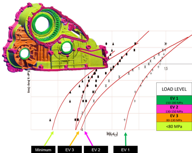
Figure 21. Statistical evaluation of the properties in different zones using a Weibull analysis of the calculated values. The curves demonstrate that the results align with statistically expected distributions. Additionally, the minimum expected properties in each zone can be inferred from the results.
