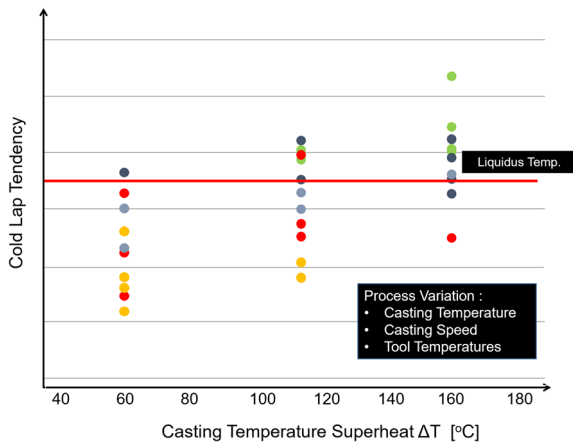
Figure 6. Systematic investigation of process variations on the tendency of cold runs with casting process simulation using a virtual test plan. Each point corresponds to the result of a simulation with different process or boundary conditions. The evaluation criterion is the liquidus temperature. In this example, the process variations investigated (casting temperature, shot time, and mold temperatures) lead to cold runs in only two out of ten variants when the melt overheats by 160 °C. At 110 °C, seven out of ten variants are at risk of being rejected, and at 60 °C, nine out of ten variants are at risk of being rejected.
