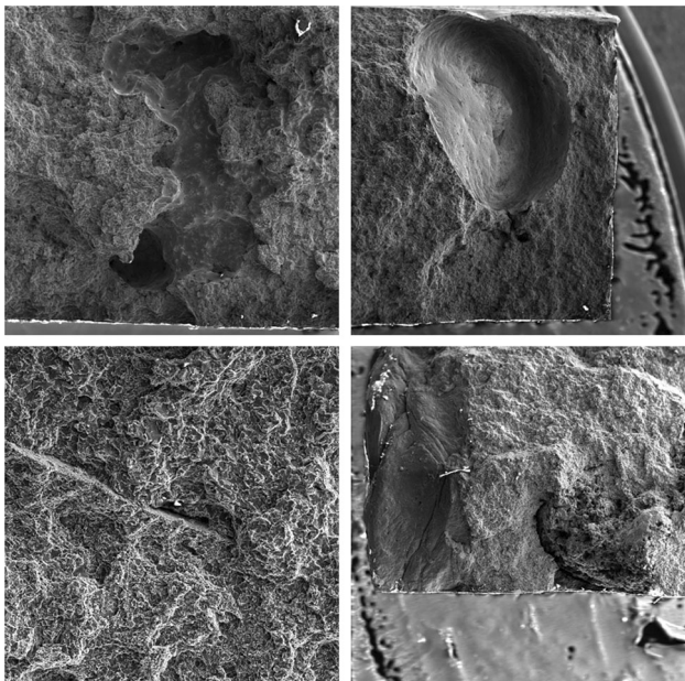
Figure 3. Typical casting defects in die casting: micro-porosity (top left), entrapped air and hydrogen precipitation during solidification (top right), oxides (bottom left), or cold running (bottom right).
