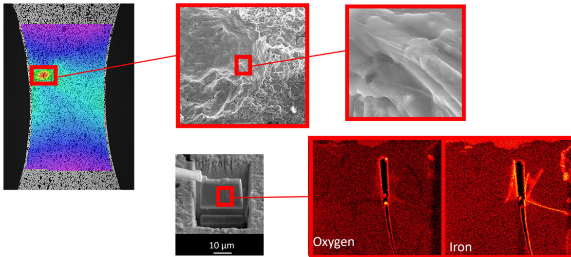
Figure 10. Determining the root cause of failure in a tensile specimen. Digital image correlation and scanning electron microscope observations of aluminum castings show that fracture is caused by an oxide layer that acts as a strain concentration under load. 29, 30
