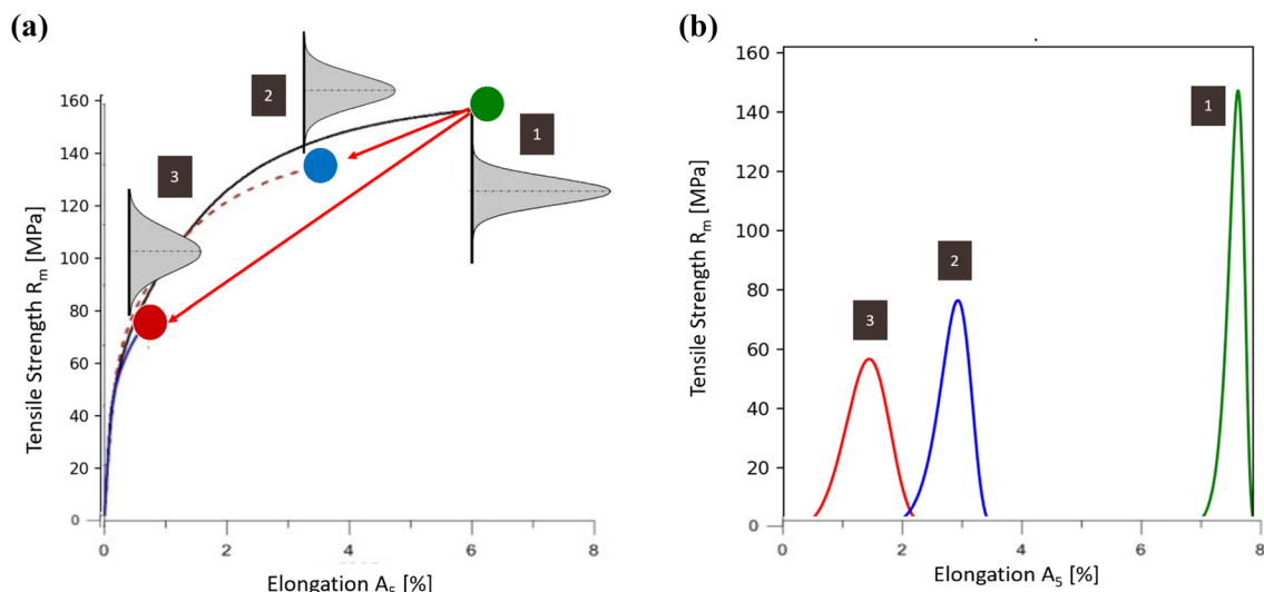
Figure 14. Calculation of total strength based on the determined defect distribution for three different locations in the part (a). Using the specified process variability, a probability function for the expected mechanical properties can be determined for each location in the casting (b).
