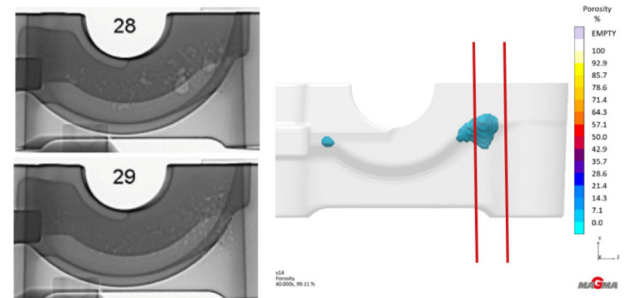
Figure 8. Comparison of simulation results with real failure patterns. The simulation shows a region, where defects occur. However, depending on the location and specification, the real defect is critical or acceptable. 28
