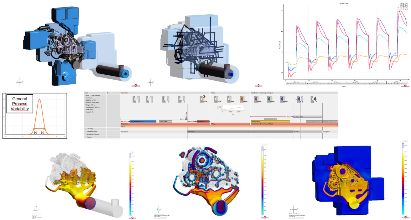
Figure 15. Specification of a process variability, the process setup and classic results of die casting process simulation: mold filling (bottom left), solidification (bottom center) and mold temperatures (bottom right) are the basis for probabilistic modeling of microstructures and properties.
