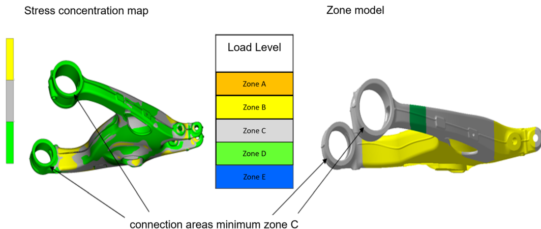
Figure 1. Technical specification for aluminum sand, gravity and die casting. Division of the component into zones of equal strength (left). A zone model is derived based on results from e.g., durability calculations, crash simulations and misuse cases. The zones tolerate different defect sizes and frequencies (right). 1
