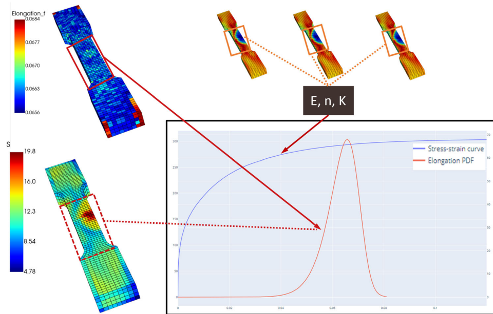
Figure 12. Distribution of calculated fracture strains A5 (top left) and their probability density function in a tensile member (bottom left). This information can be represented in a stress–strain curve and a probability density function and made available to other calculation programs with a few parameters ( E , n , K ).
