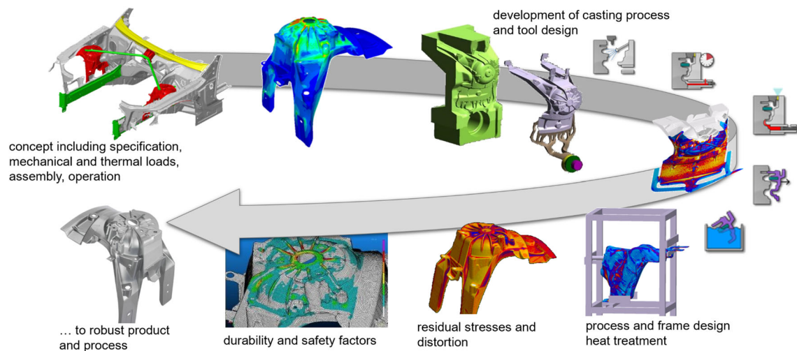
Figure 5. Integrating casting process simulation results into product development and process design.
