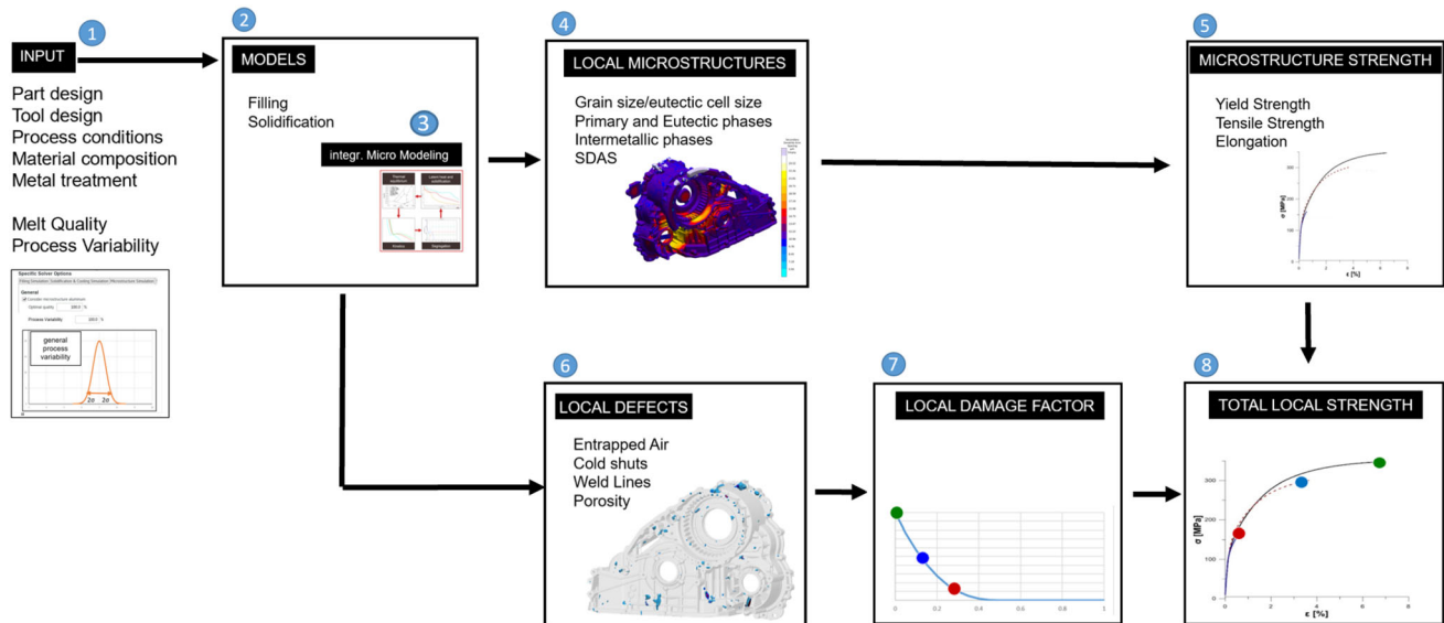
Figure 13. Flow chart of the core process of the methodology for a calculated design
